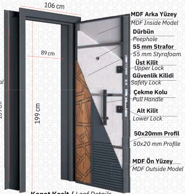
Kanat Kesit / Leaf Details
