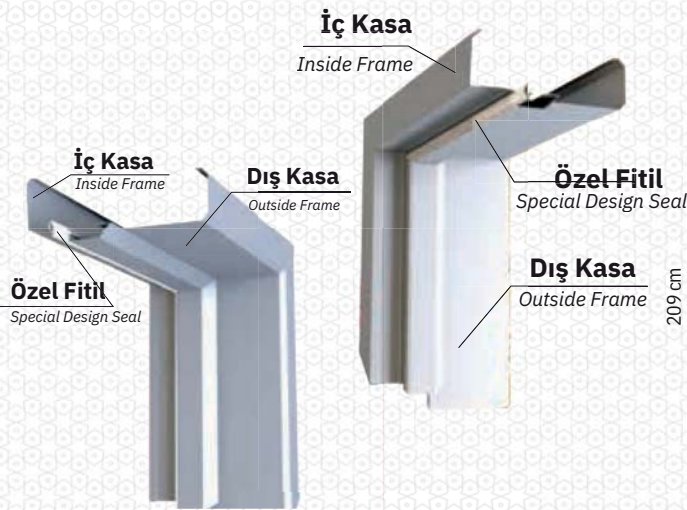
Kasa Kesit / Frame Details
